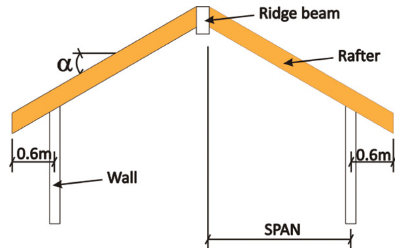
Figure B. Rafter Loading
